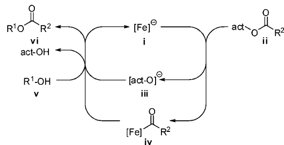
Figure 2. Mechanistic proposal.
